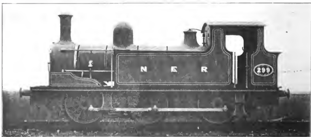
Fig. 5029. Six-Coupled Tank Shunting Locomotive. North Eastern Railway. Cylinders 16 in. x 22 in.; Total Heating Surface 731 sq. ft.; Diameter of Drivers 55 1/2 in.; Weight on Drivers 82,160 lbs.; Total Weight 82,160 lbs.
